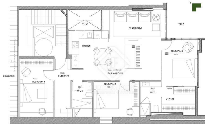
APARTMENT OP. 1 102,38qsm (livable area) 115,17qsm (constructed area)
