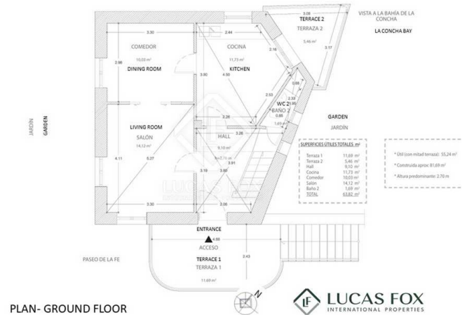
PLAN- GROUND FLOOR
