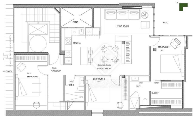
APARTMENT OP. 2 102,28sqm (livable area) 115,17sqm (constructed area)
